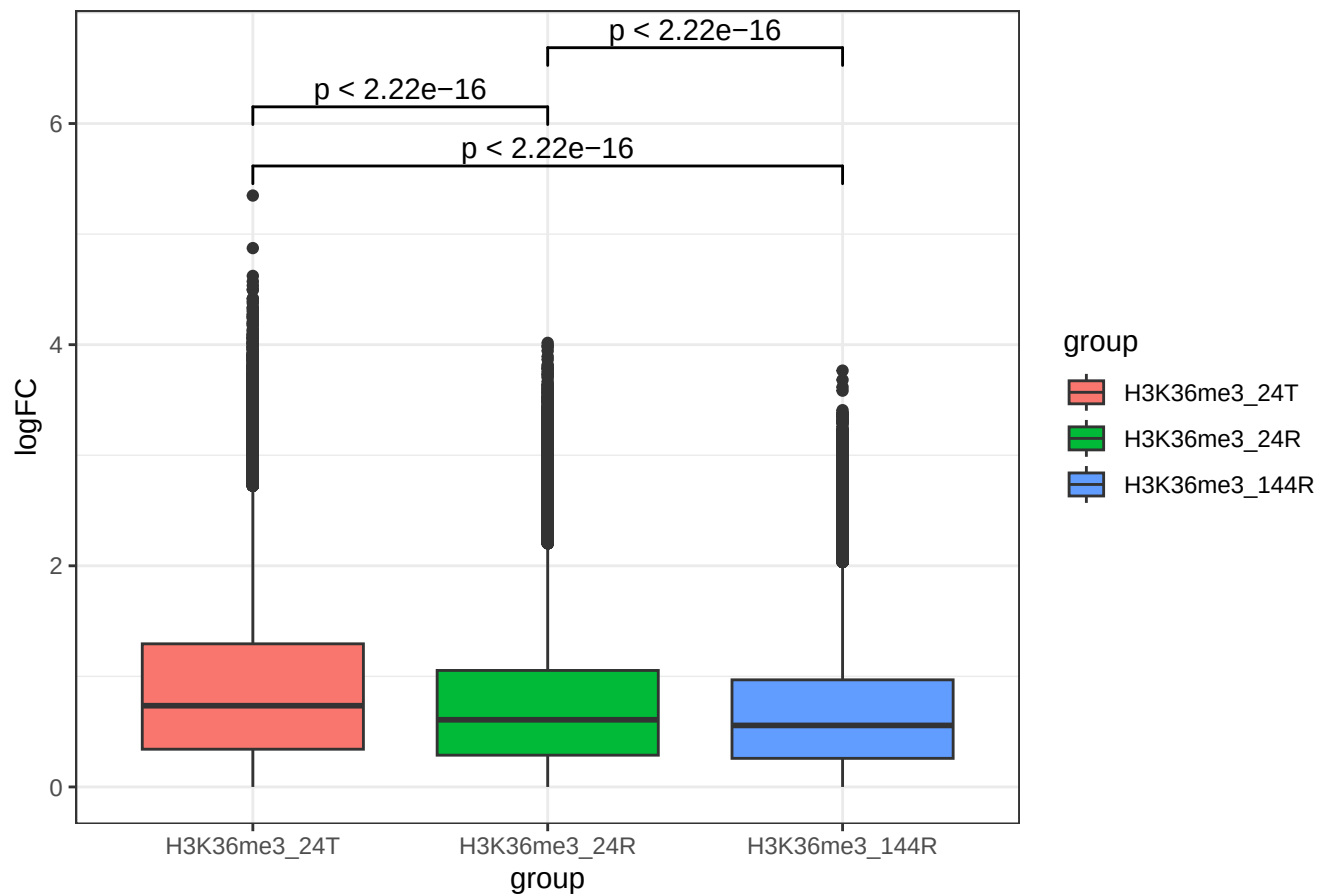
Absolute LFC across time for H3K36me3
